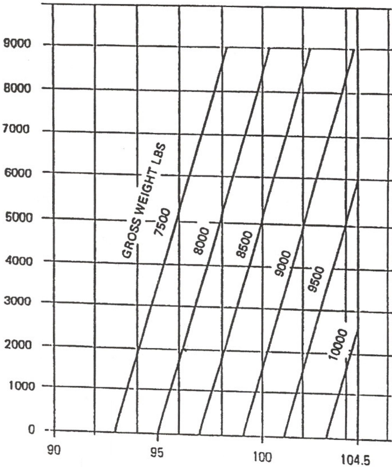
AUTOROTATION CALLIBRATION CHART BELL 205 A-1 with 212 BLADES / BELL 212
